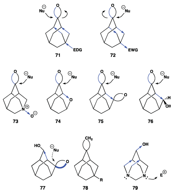
Fig. 29 Preferred stereoselectivity on rigid tricyclic frameworks.
