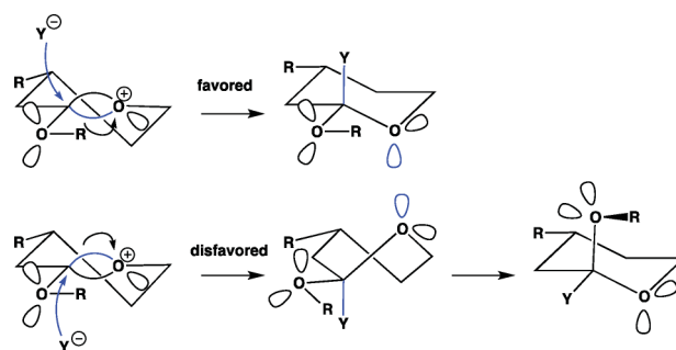
Fig. 19 Reaction of alkoxy-carbenium ion with nucleophiles.
