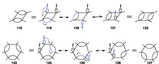
Fig. 37 Cyclobutadiene and benzene.
