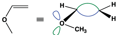
Fig. 9 Preferred s-cis conformation for methyl vinyl ether.
