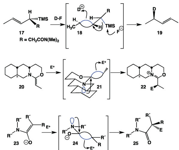
Fig. 13 Preferred anti reactivity in a series of SE'-related reactions.
