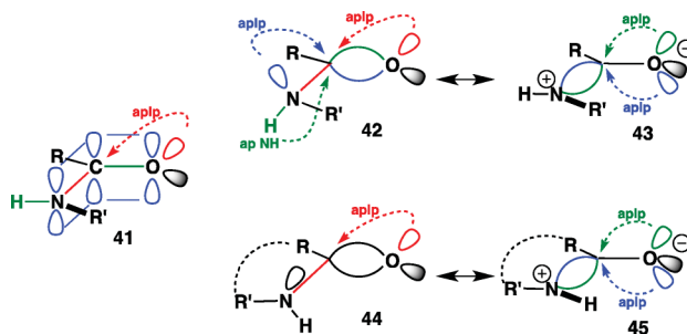
Fig. 20 \sigma/\pi (left) and bent bond models (right) of 2° amides.
