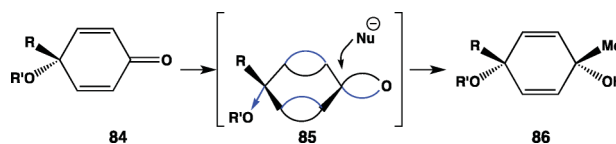
Fig. 31 Nucleophilic addition to cyclohexadienone derivatives.
